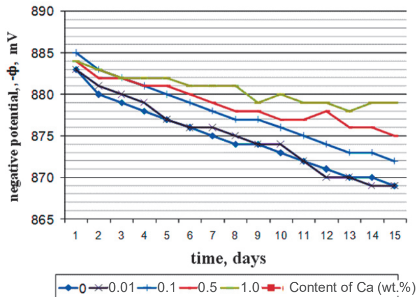
Fig. 1 Change stationary potentials AP1 alloy samples (with a change in the Ca content of 0 to 1.0 wt.%)
