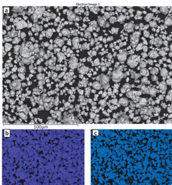
Fig. 3 SEM images of powder for 10 hrs of 400 RPM milling, 15 mm balls b) Cr map c) Fe map
