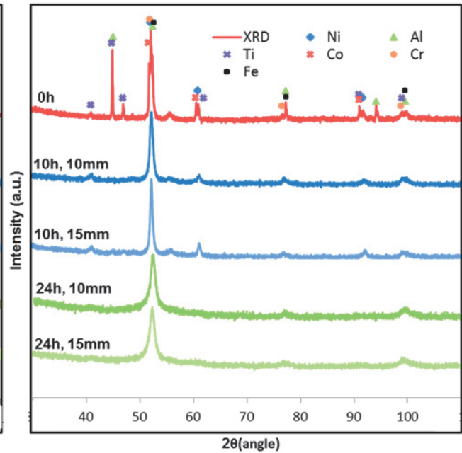
Fig. 2 XRD results of AlCoCrFeNiTi 0.5 powders after different milling times and balls diameters at 250 RPM
