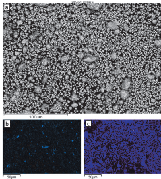
Fig. 6 SEM images of powder for 24 hrs of 250 RPM milling, 15 mm balls b) Cr map c) Fe map
