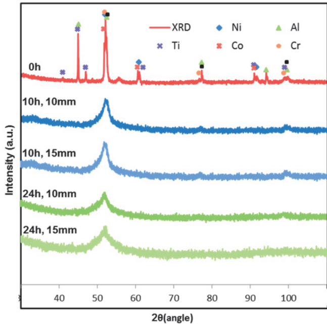
Fig. 1 XRD results of AlCoCrFeNiTi 0.5 powders after different milling times and balls diameters at 400 RPM
