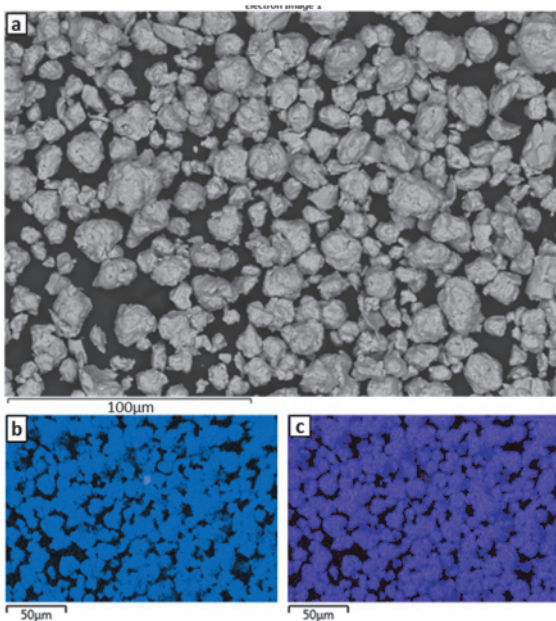
Fig. 5 SEM images of powder for 24 hrs of 400 RPM milling, 15 mm balls b) Cr map c) Fe map
