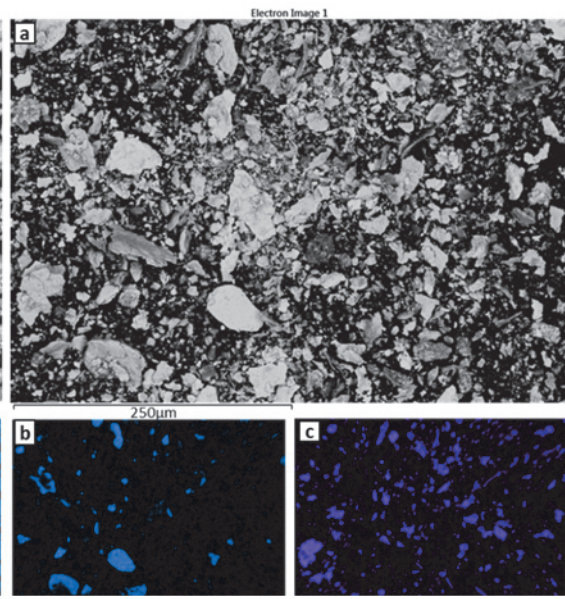
Fig. 4 SEM images of powder for 10 hrs of 250 RPM milling, 15 mm balls b) Cr map c) Fe map
