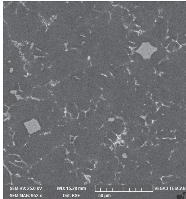
Fig. 7 Detail of light iron-copper phase at dendrite boundaries and light iron-manganese sharp particles in BSE mode
