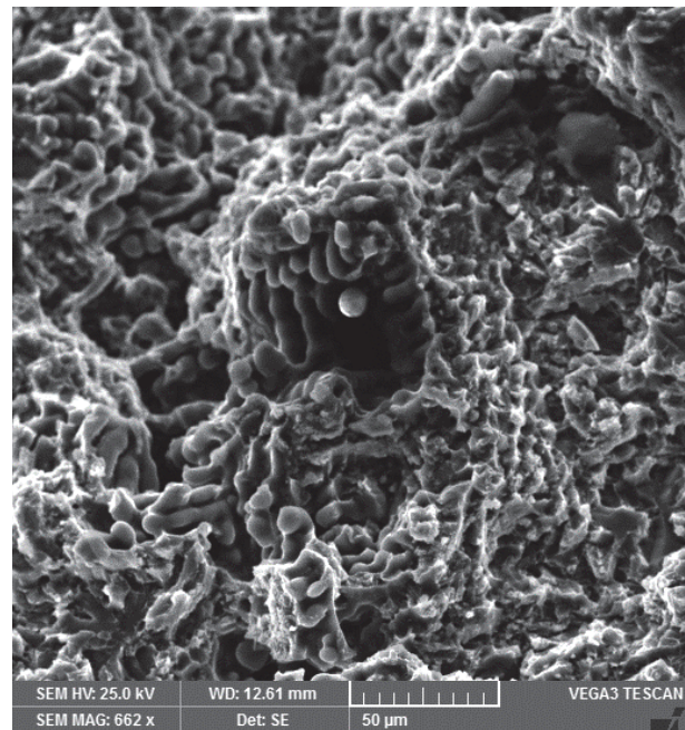
Fig. 9 Dendrites on the fracture surface
