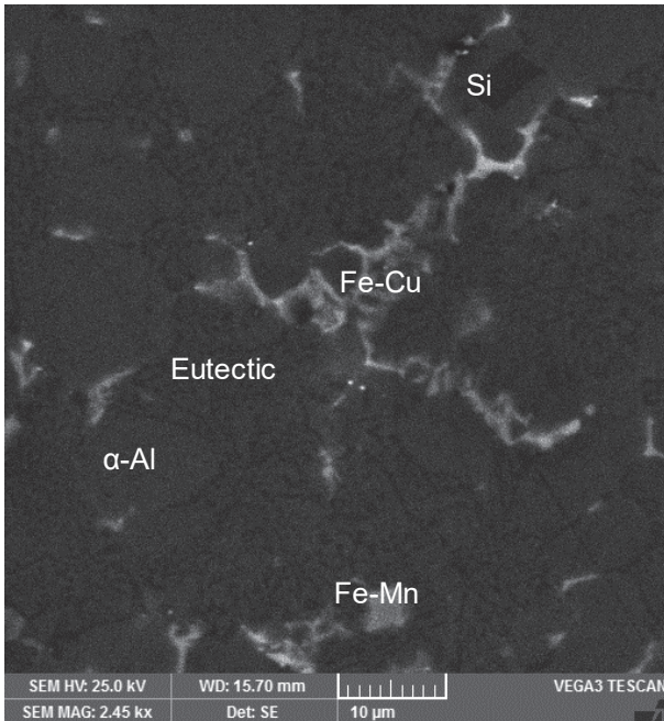
Fig. 6 Dendritic microstructure of the fork with interdendritic eutectic network, particles at dendrite boundaries (Fe-Cu) and two kinds of larger particles inside dendritic areas (primary Si and Fe-Mn)
