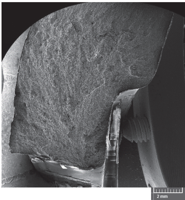
Fig. 8 Fracture initiation area at the surface of the fork, larger shrinkages visible.
