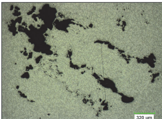
Fig. 4 Large shrinkage in material
