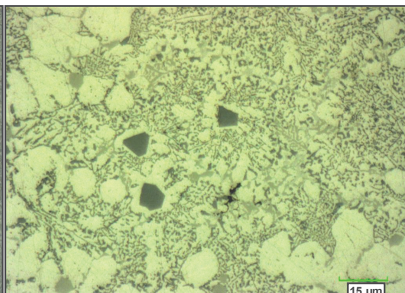
Fig. 5 Dendritic microstructure with eutectic network and several kinds of particles
