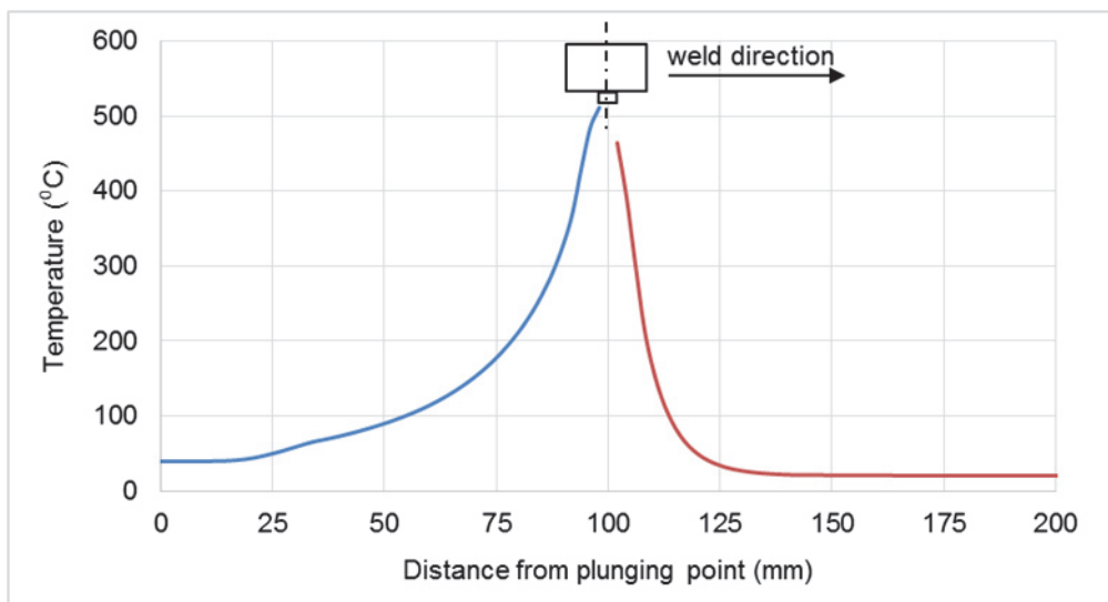
Fig. 5 Maximum temperature distribution along the weld centreline
