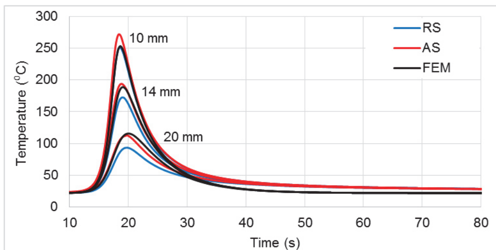
Fig. 7 Comparison of calculated and measured temperature cycles
