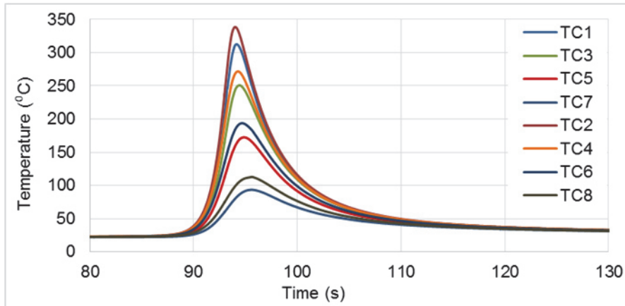
Fig. 2 Temperature cycles during FSW at 710 rpm
