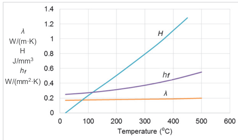
Fig. 4 The thermophysical properties of workpieces material
