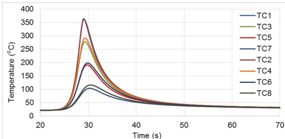
Fig. 3 Temperature cycles during FSW at 1120 rpm
