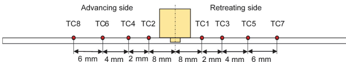
Fig. 1 Thermocouples position
