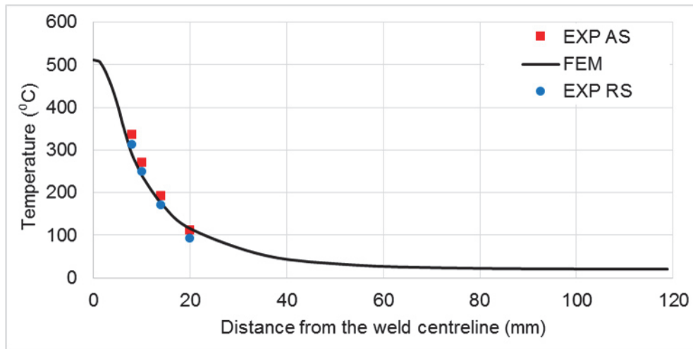
Fig. 6 Comparison of numerical maximum temperature distribution and measured value
