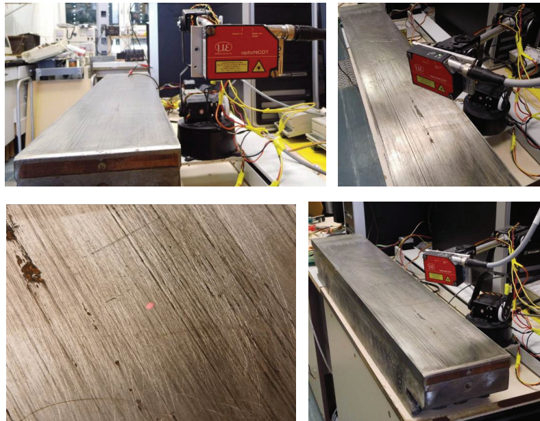
Fig. 4 View of the measuring assembly for verification of the surface - the wear surface metallurgical materials (measurements in laboratory conditions VSB - Technical University of Ostrava)
