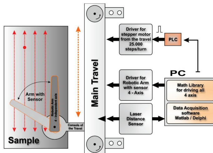
Fig. 3 The principle of scanning the surface of the mold using a robotic arm with a laser sensor
