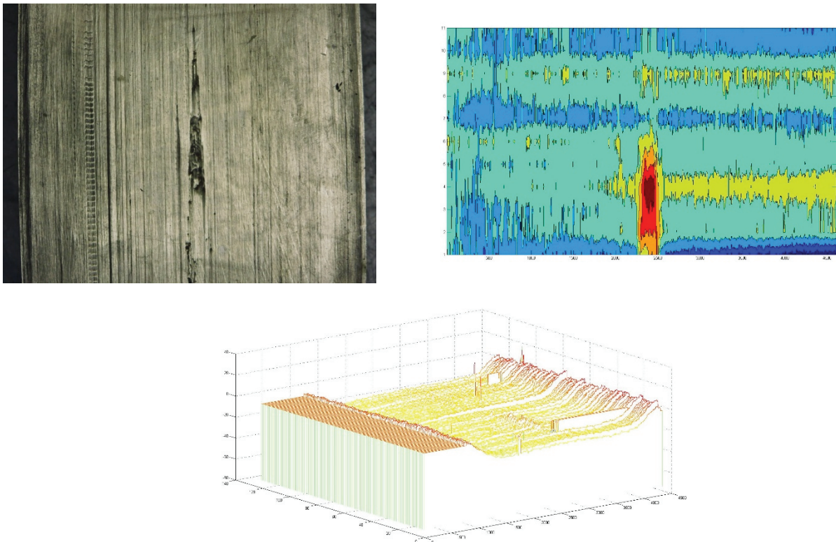
Fig. 5 Demonstration of results visualization surface metallurgical materials (original surface, 2D visualization with filter, 3D visualization)
