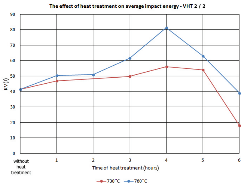
Fig. 3 The effect of heat treatment on average impact energy - VHT 2 / 2
