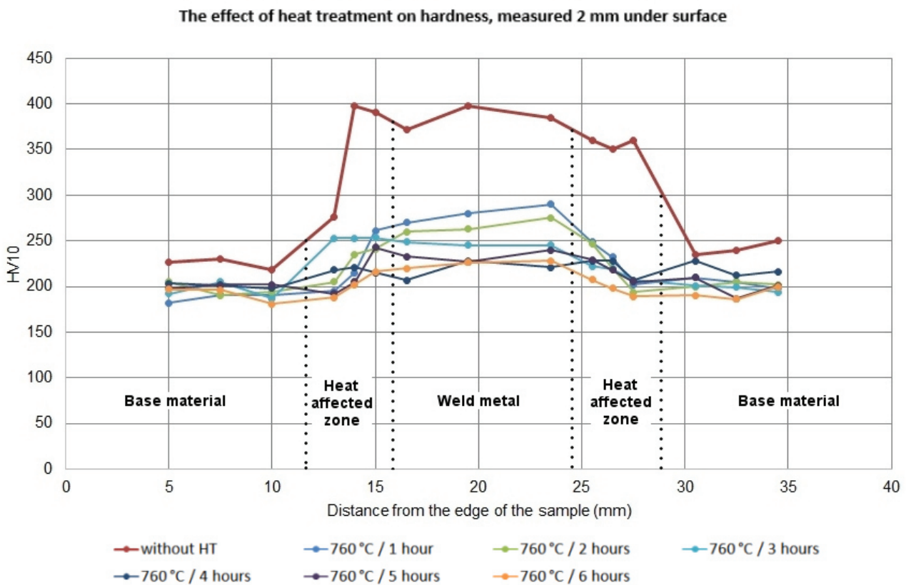
Fig. 4 The effect of heat treatment on hardness
