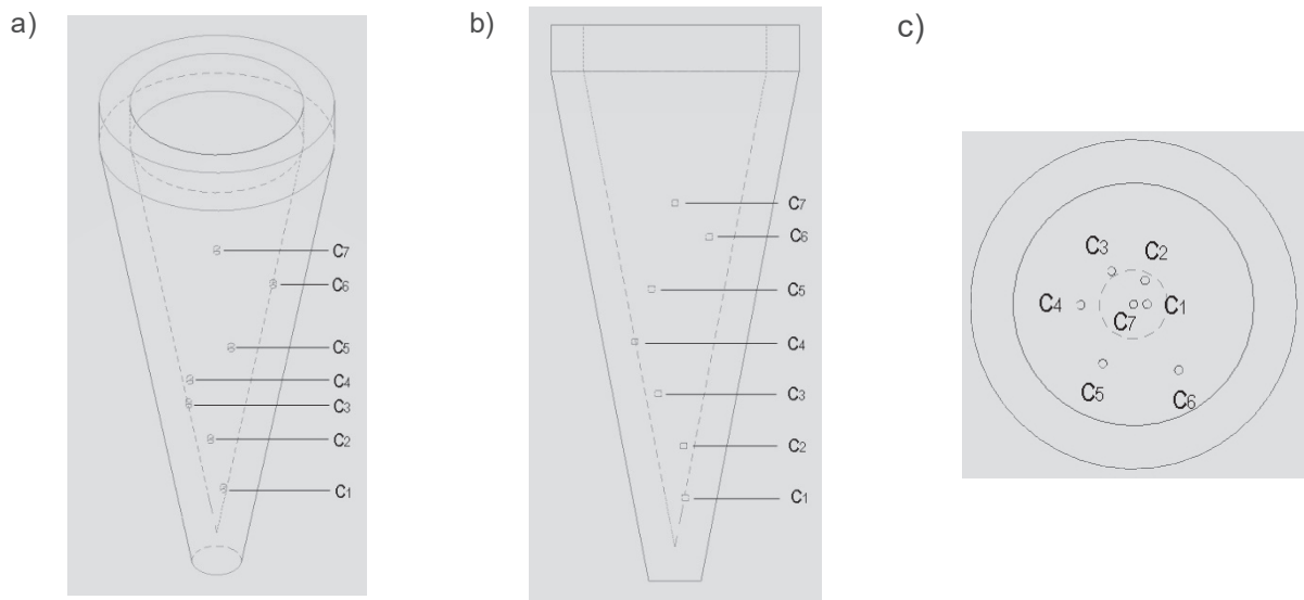
Fig. 1 Examples of arrangement of sensors C1 ÷ C6 in the mould enclosing cone experimental casting. C7 sensor is located in the geometric centre of the experimental casting
