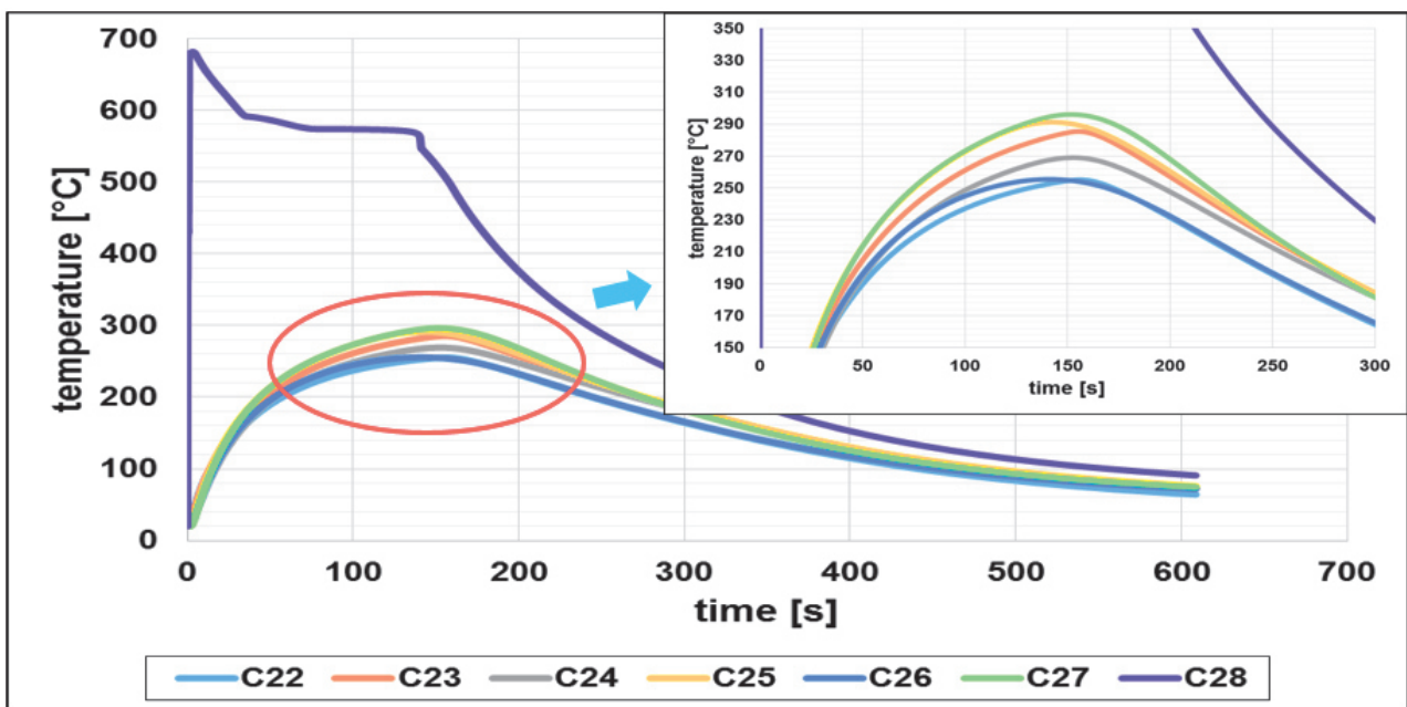
Fig. 5 Temperature change in 6 mm from casting surface distance
