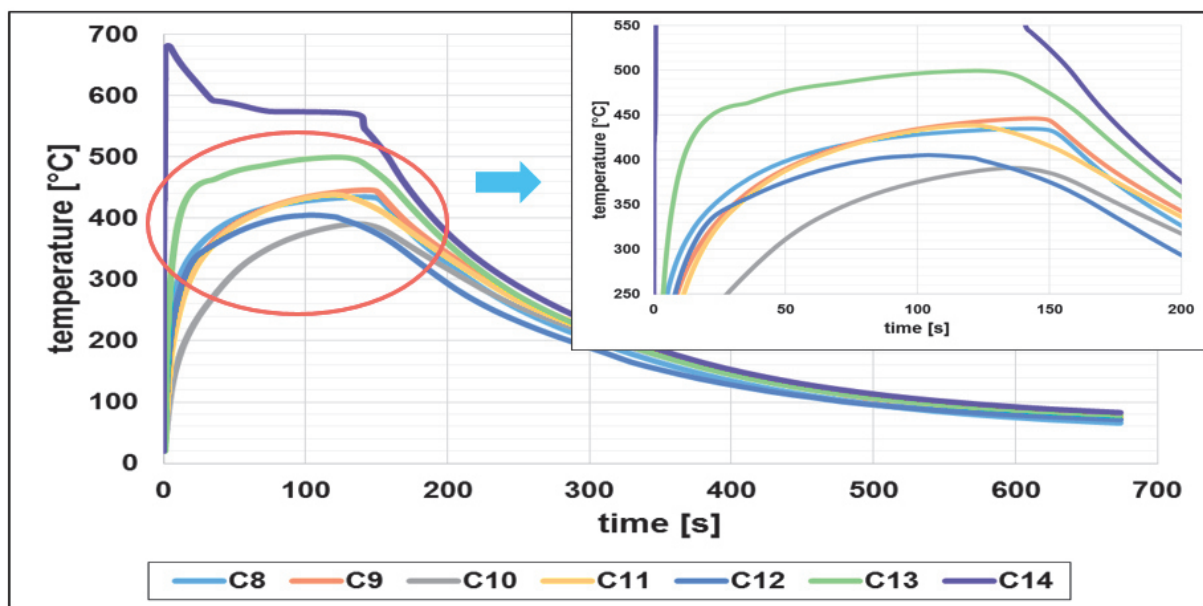
Fig. 3 Temperature change in 2 mm from casting surface distance
