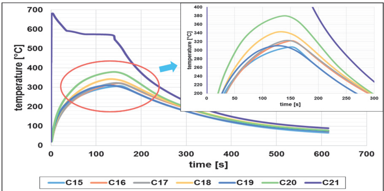
Fig. 4 Temperature change in 4 mm from casting surface distance
