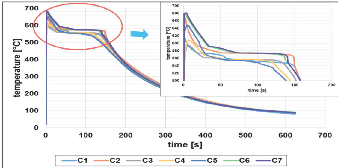
Fig. 2 Temperature change at the mould-casting contact
