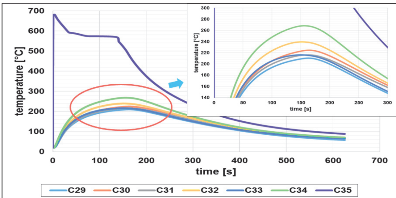
Fig. 6 Temperature change in 8 mm from casting surface distance
