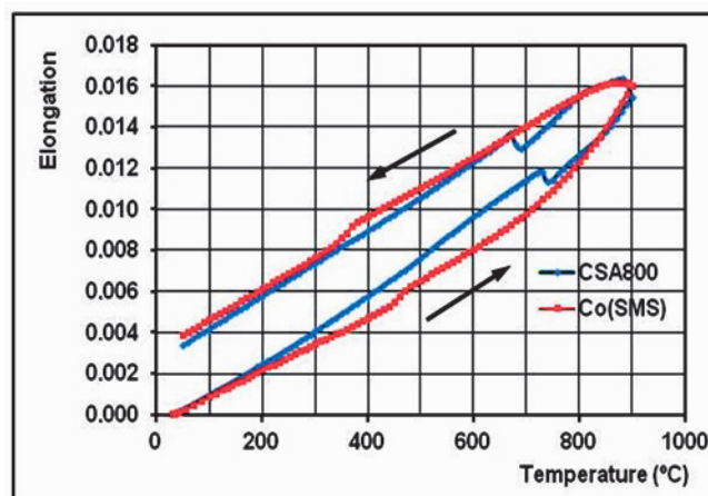
Fig. 3 Dimensional changes in the CSA800 and Co (SMS) sinters detected by dilatometry
