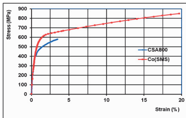
Fig. 2 Comparison of the tensile strength curves for the CSA800 and Co (SMS) sinters
