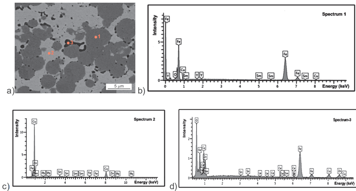
Fig. 5 Microstructure of the CSA800 sinter (a) with the X-ray spectra for the particular phases (b, c, d)
