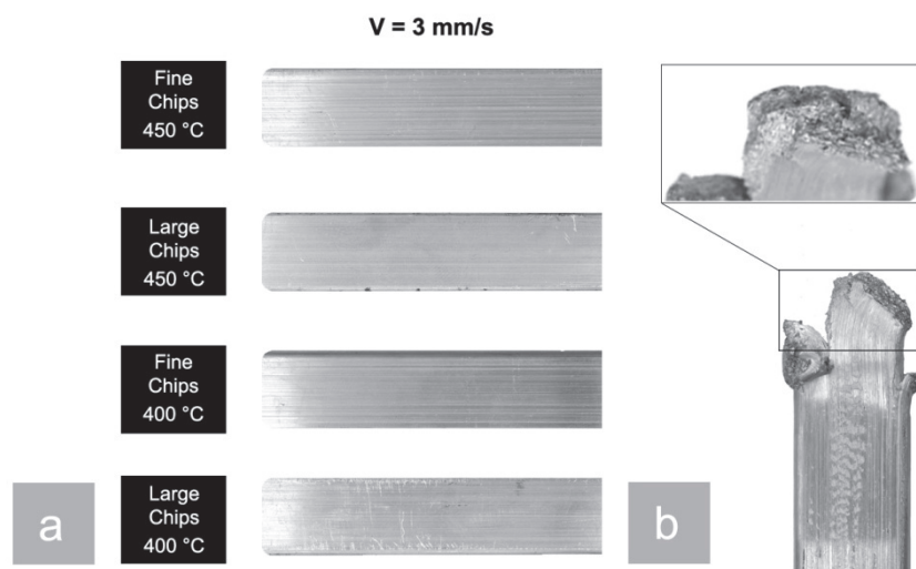
Fig. 3 a) Surfaces of as-extruded profiles b) “transition zone”
