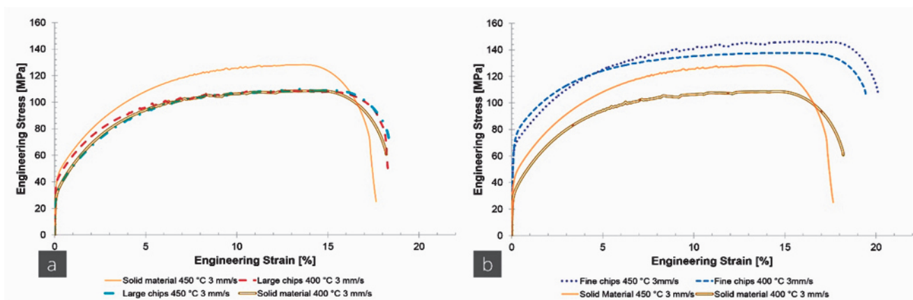
Fig. 4 Engineering stress-strain curves for exemplary samples extruded from a) large chips, b) fine chips
