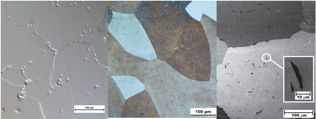
Fig. 1 The structure of alloy 1 (Fe 30 Al 3.7 Cr 0.3 Zr 0.2 C) [10]
