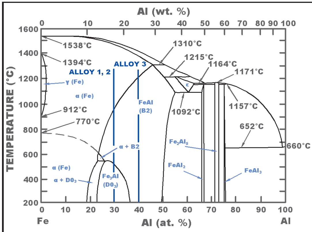
Fig. 5 The binary Fe - Al diagram with marked composition of investigated alloys
