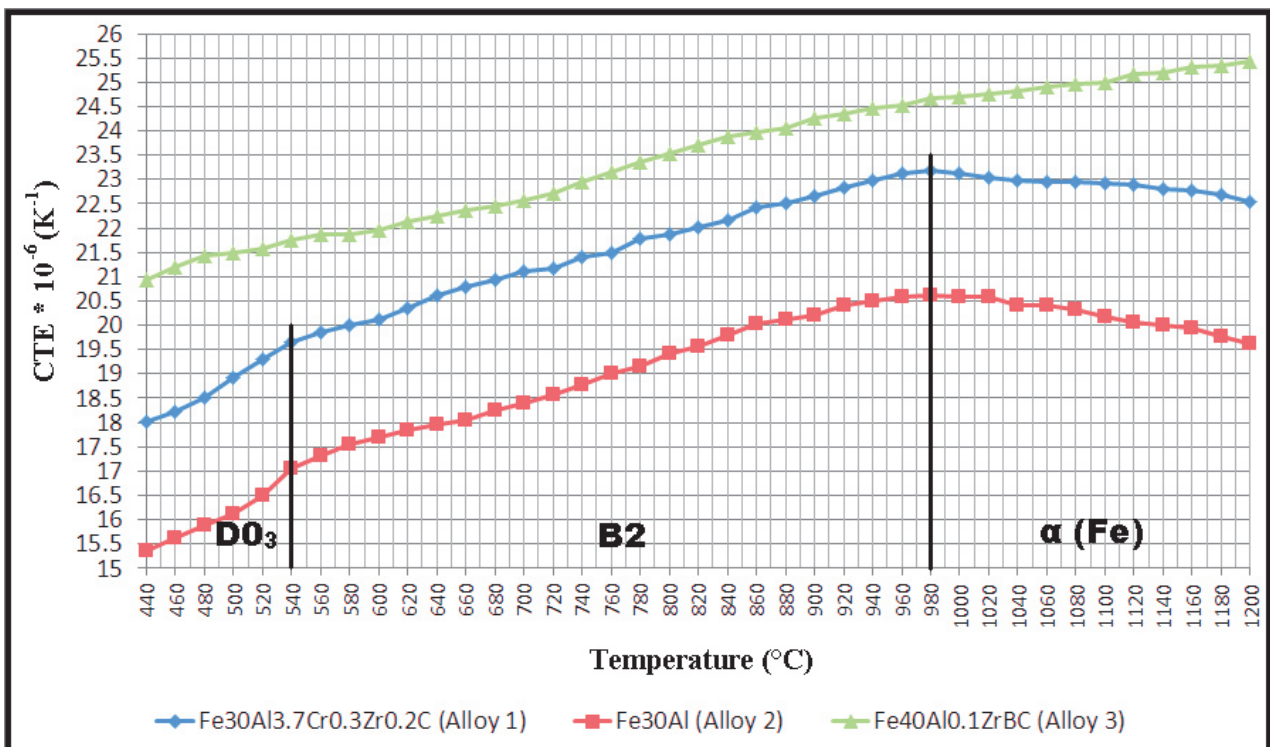
Fig. 4 The CTE chart of investigated alloys
