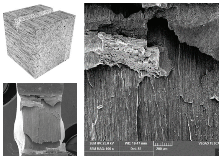
Fig. 4 The 3D reconstruction of texture MA957 and fracture surface of mini Charpy specimen exposed to He 720 °C and impact tested at -80 °C
