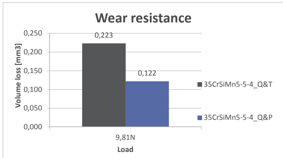
Fig. 2 Volume loss of the samples after sliding friction
